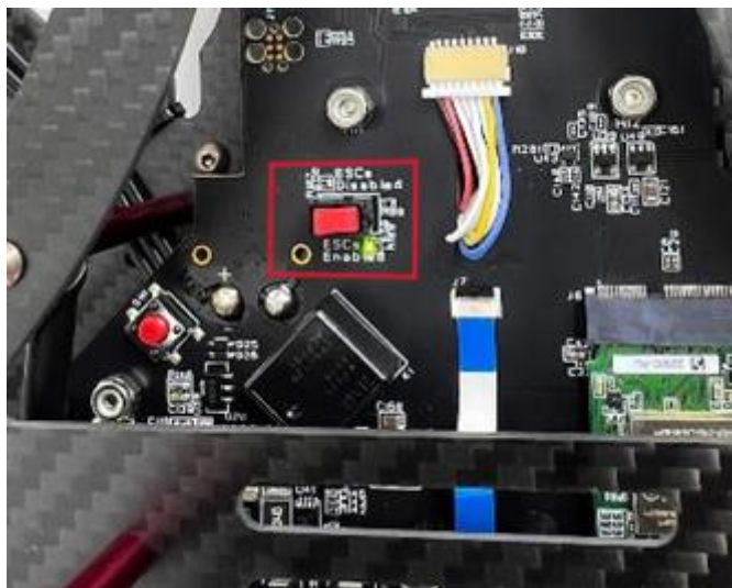
Figure 4 ESCs Enable Switch on QDrone2
